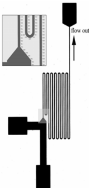
Figure .2. Schematic of 14 cm long flow chamber. Channel is 100 μm wide.
